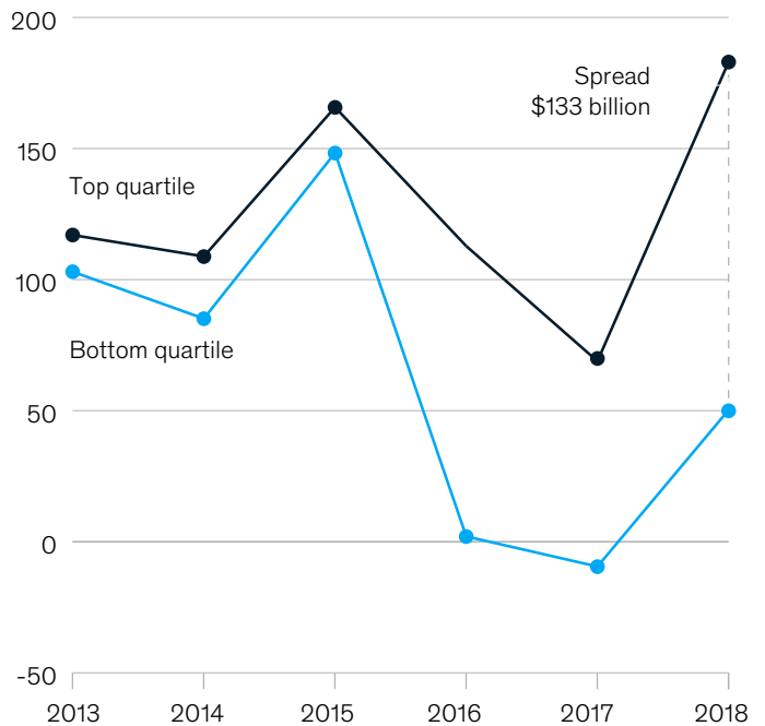
FCF, $ billion
